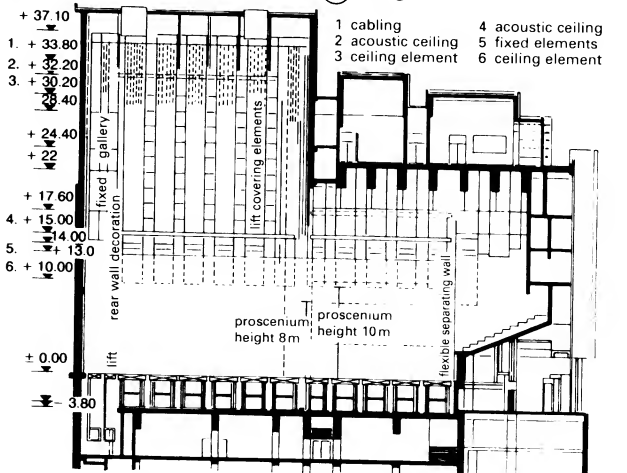
⑫ Salle Modulable, Opéra Bastille, Paris (longitudinal section)
